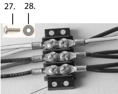
30. Terminal block
